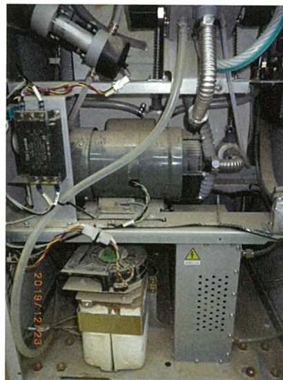
写真2：機械下側
